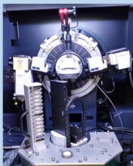
Bruker D8 XRD with Energy Sensitive Strip Detector and 30 sample auto-changer
